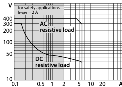
Fig. 6: Output relay load curve
