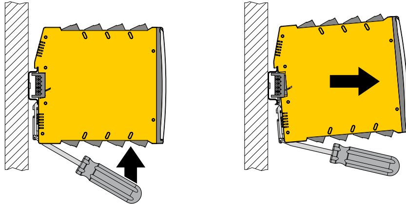
Fig. 7: Remove device
