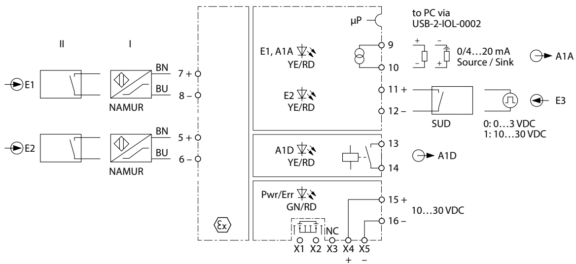
Fig. 14: Block diagram IMX12-FI01-1SF-1I1R
